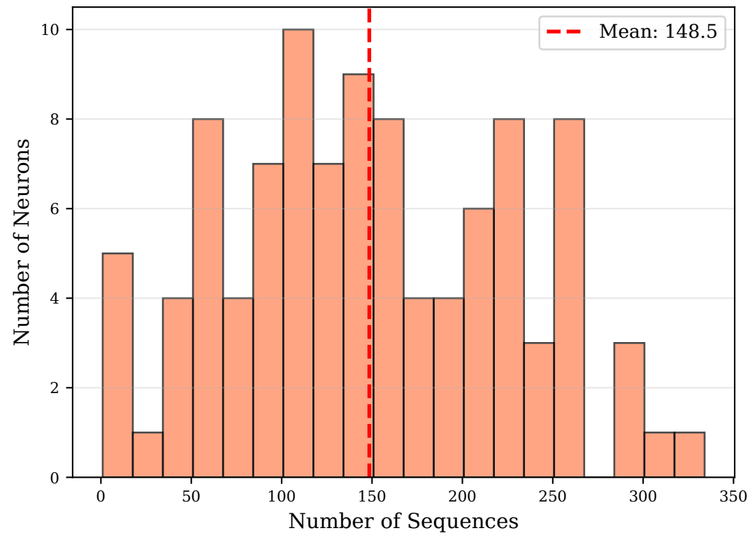
Neuron Participation - Downsampled
